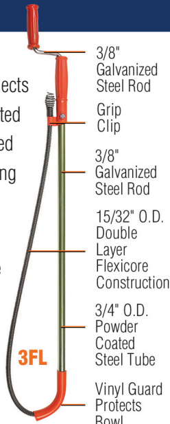
Double Spring Construction
